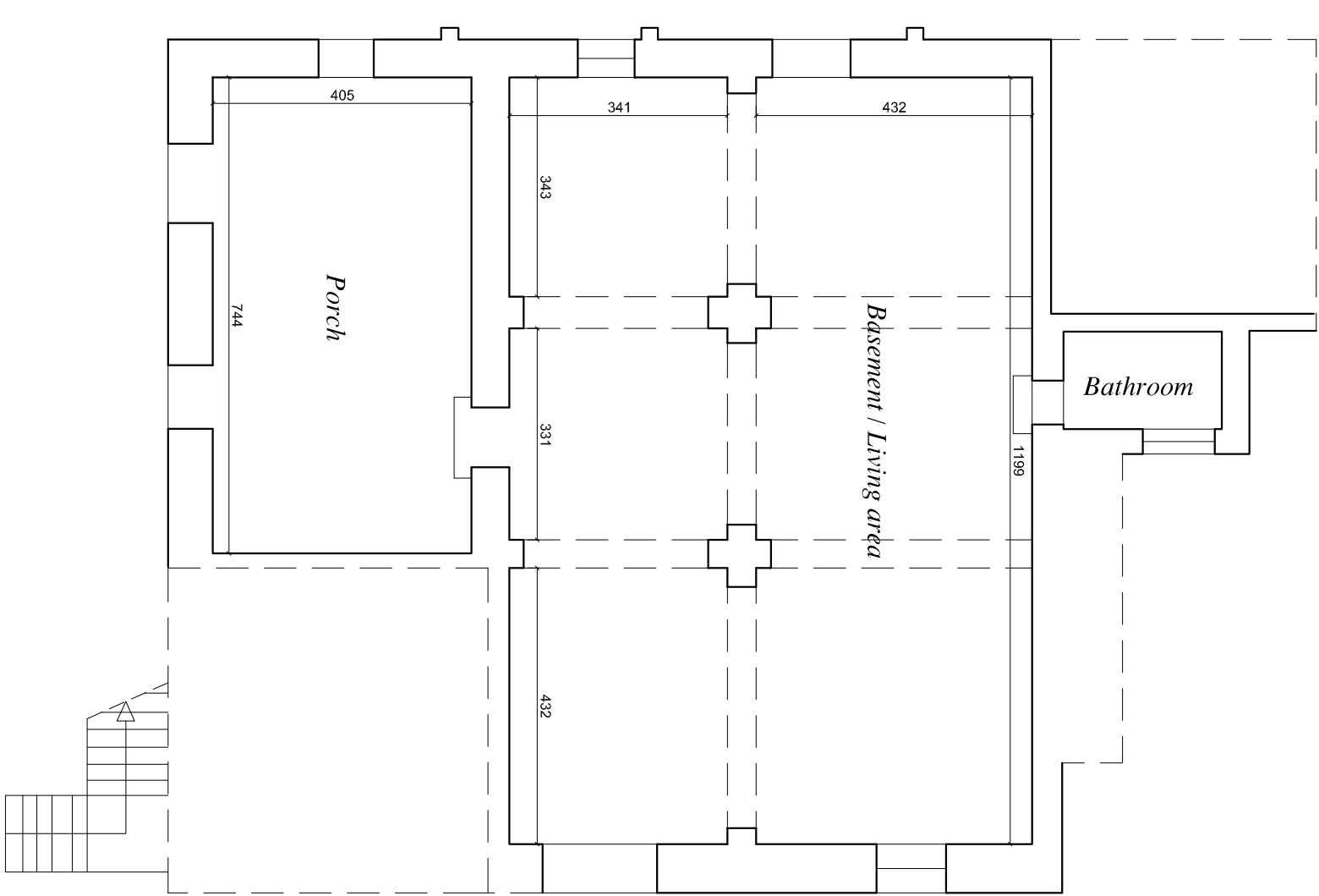
Ground floor
