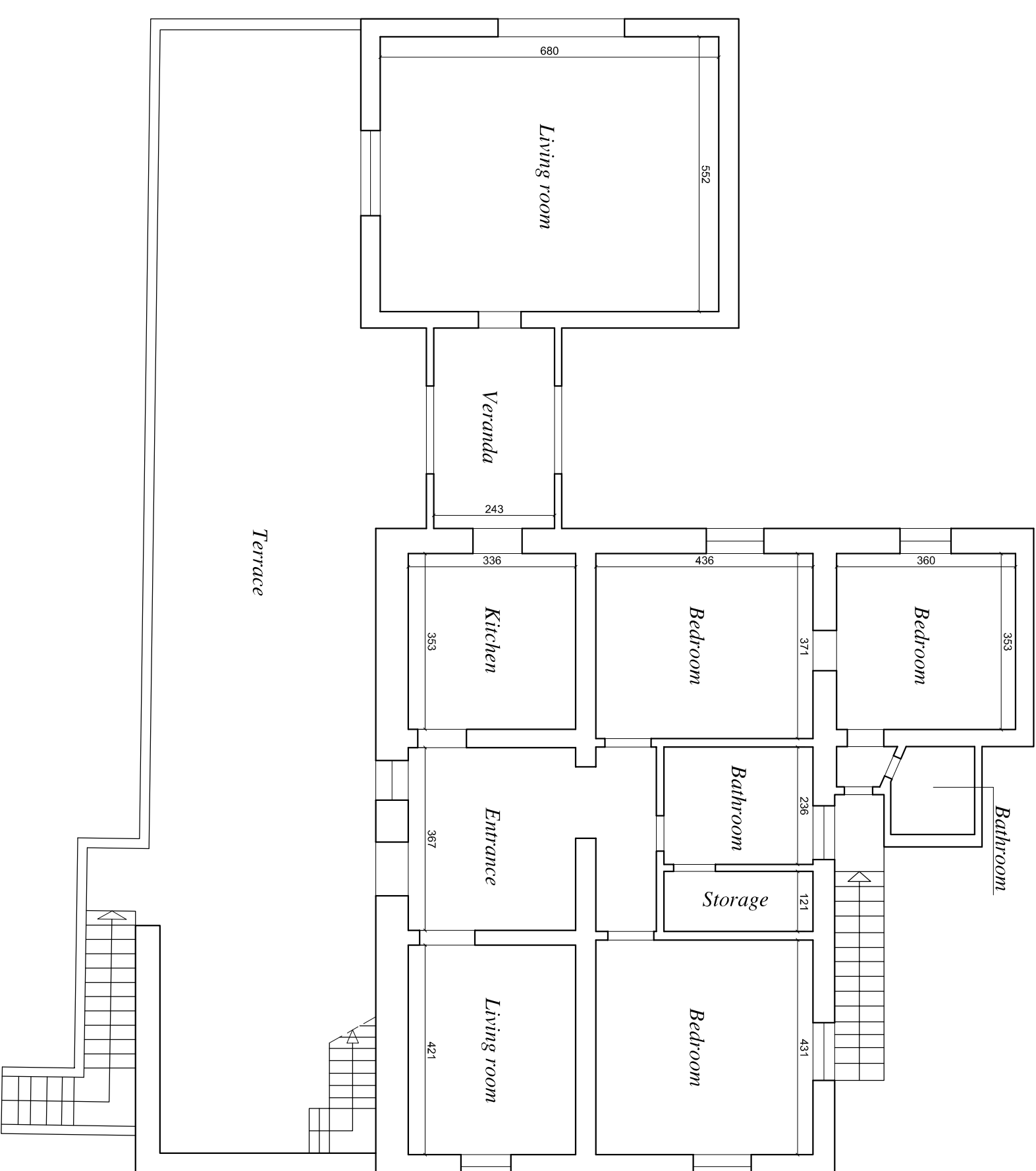
First floor
