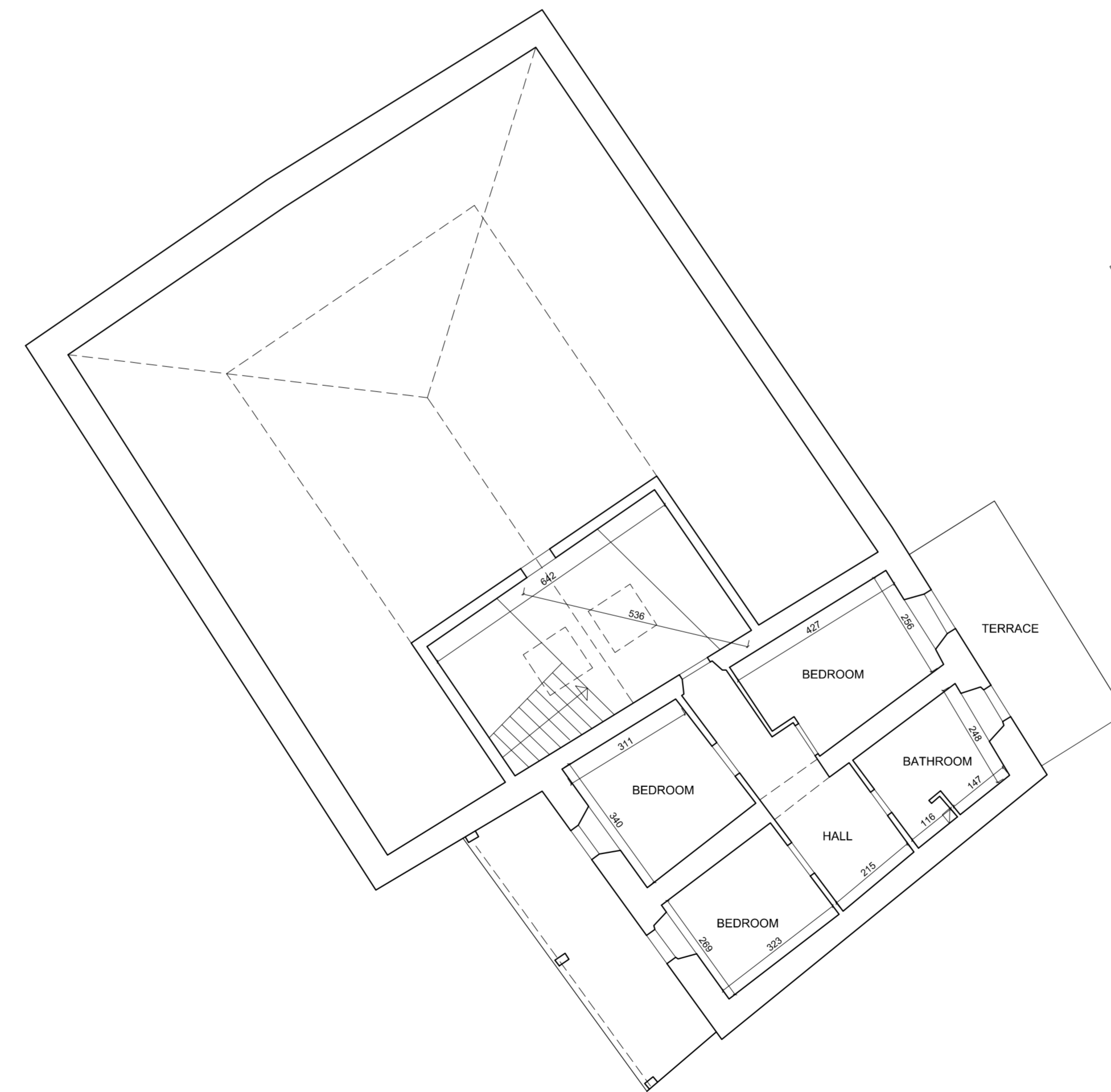
FIRST FLOOR
