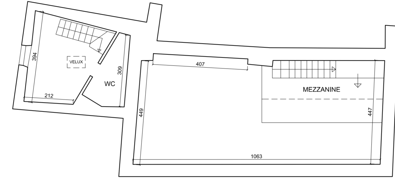
FIRST FLOOR
