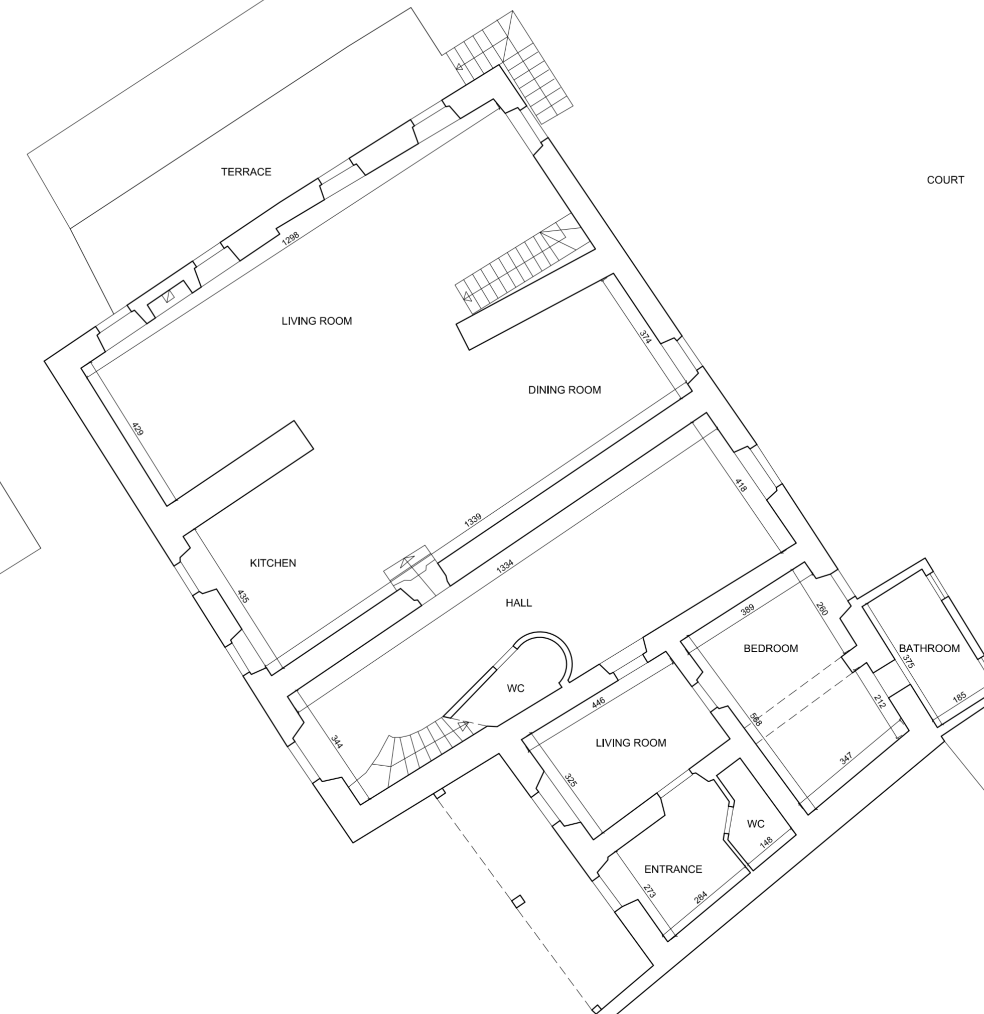
GROUND FLOOR
